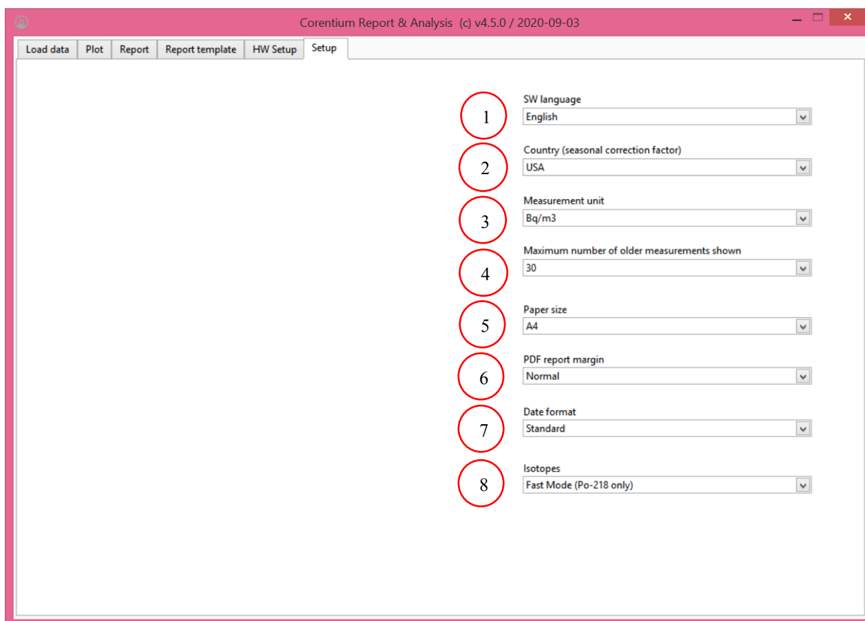
Figure 4-44 : Setup TAB - CRA SW settings
