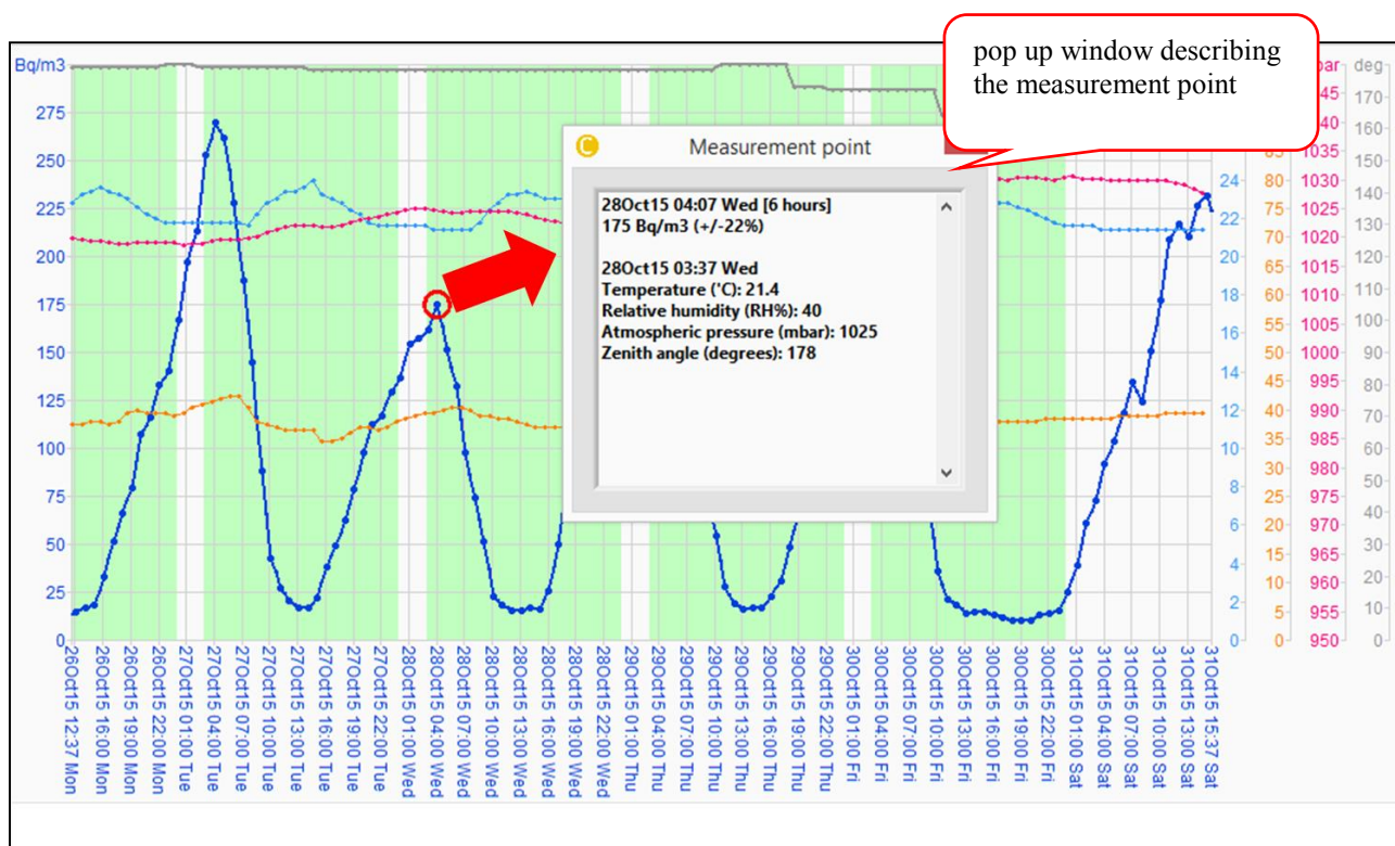
Figure 4-19: Plot TAB-Reading individual measurement point
